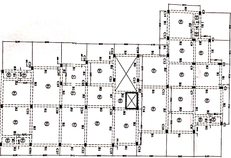
LAYOUT PLAN (BEAM & SLAB) SCALE = 1:100
